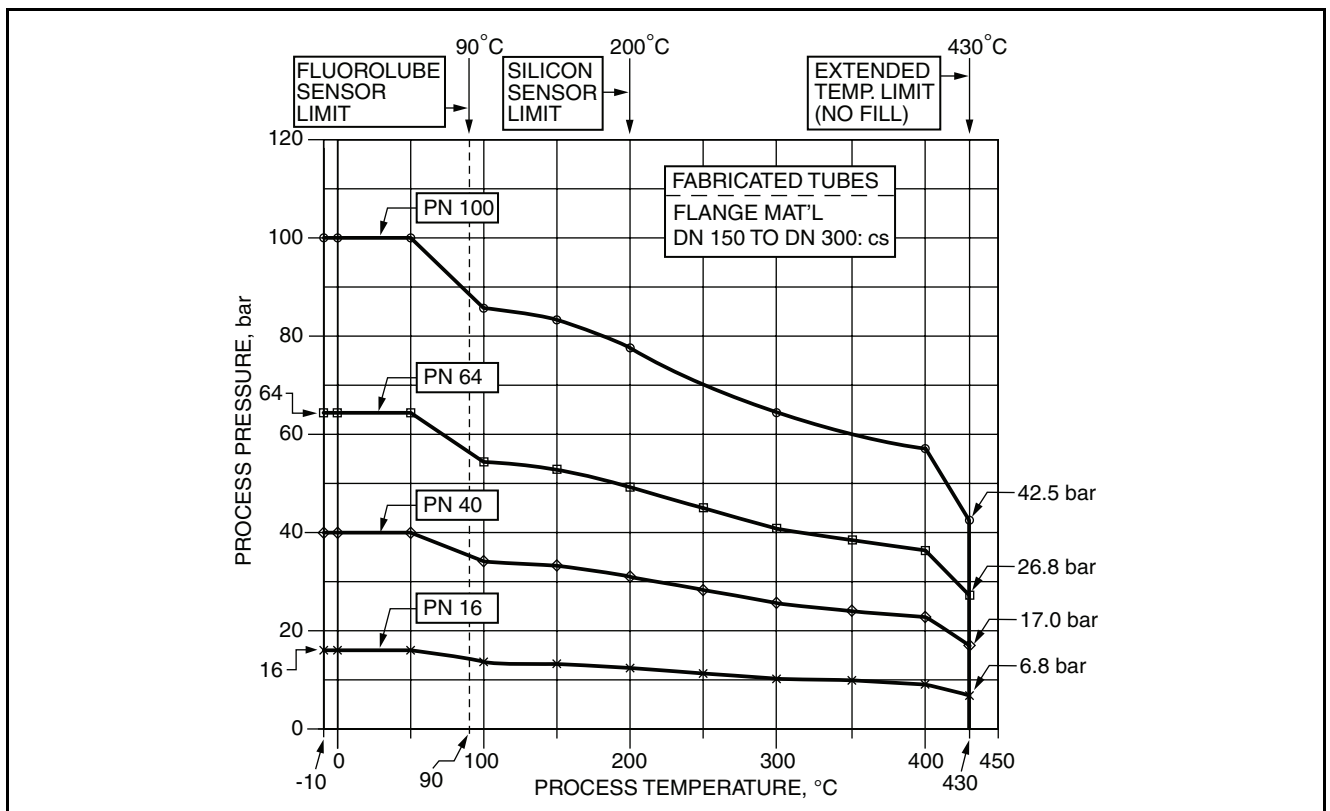
Figure 8. Metric Flange Ratings; Material Group 3E0
