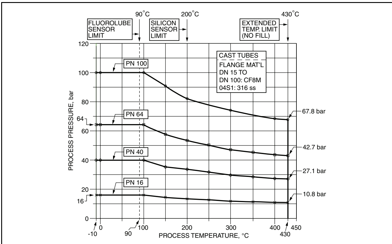
Figure 6. Metric Flange Ratings; Material Group 14E0
