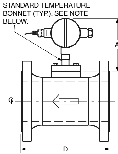
83F FLANGED BODY
