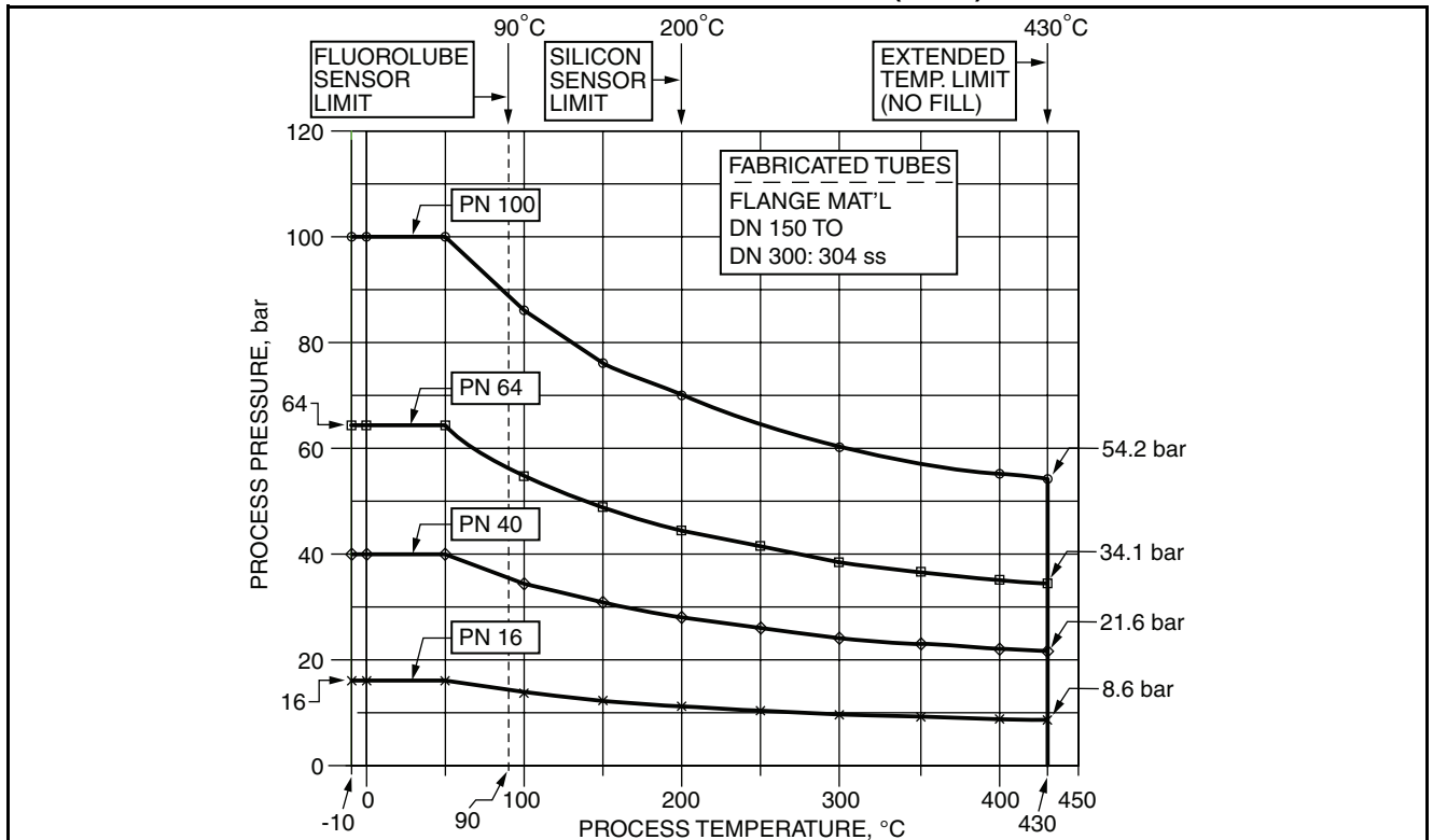
Figure 7. Metric Flange Ratings; Material Group 10E0
