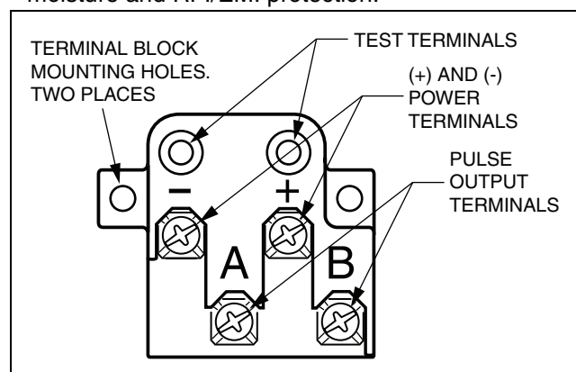
Figure 10. Terminal Block
