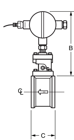
83W WITH ISOLATION VALVE
